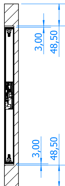
SECTION B-B
